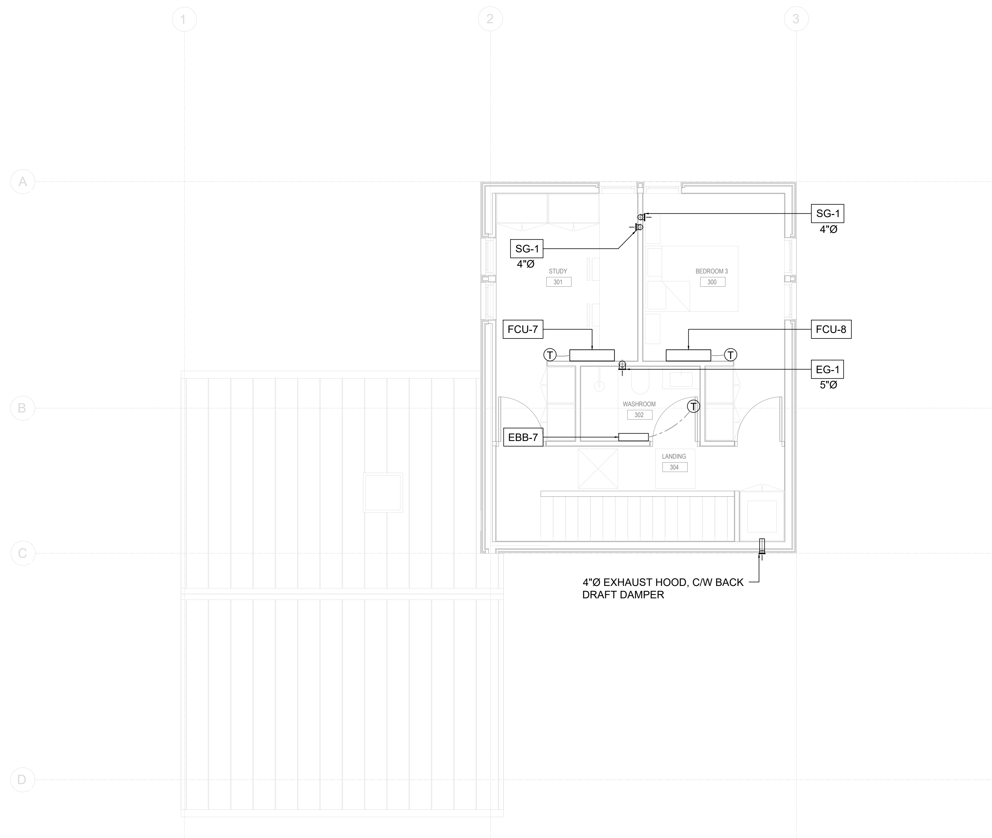
M3 1 LEVEL 3 FLOOR PLAN 1/4" : 1'
