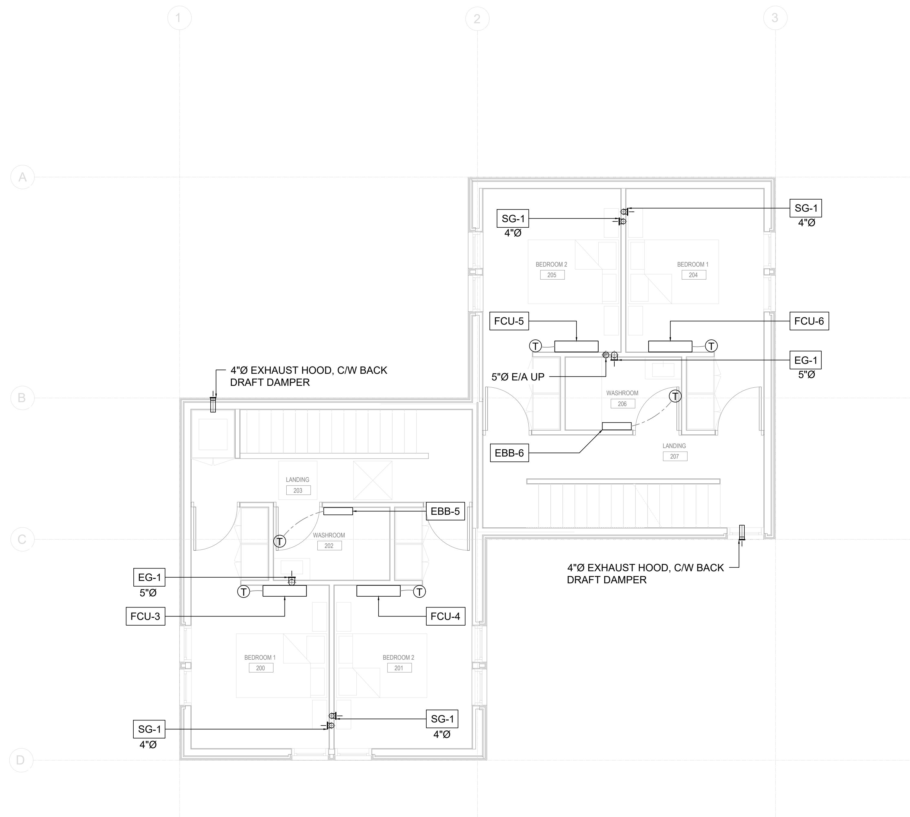
M2 LEVEL 2 FLOOR PLAN 1 1/4" : 1'
